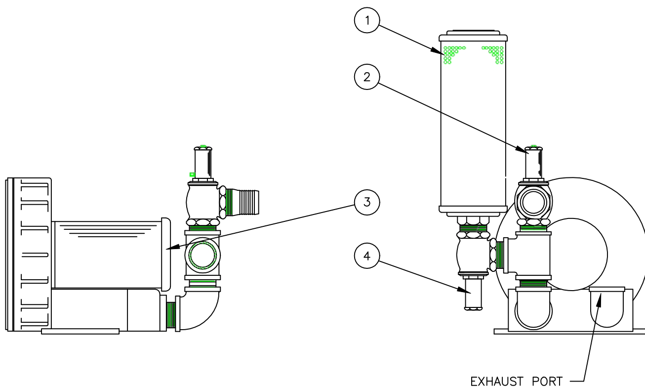
VACUUM BLOWER DETAIL
